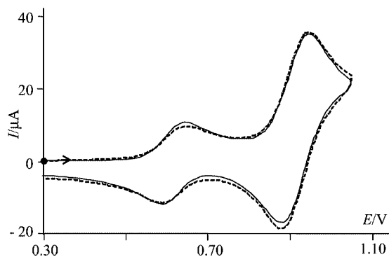
Figure 3. Cyclic voltammograms of a 0.14 mM solution of [\{\text{Ru}(\text{LL}_4)\}_3\text{Fe}\}^{8+} in \text{CH}_3\text{CN} + 0.1 \text{ M Bu}_4\text{NClO}_4 at a platinum electrode; scan rate 200 \text{ mV s}^{-1} : (---) experimental curve, (—) fitted curve.
