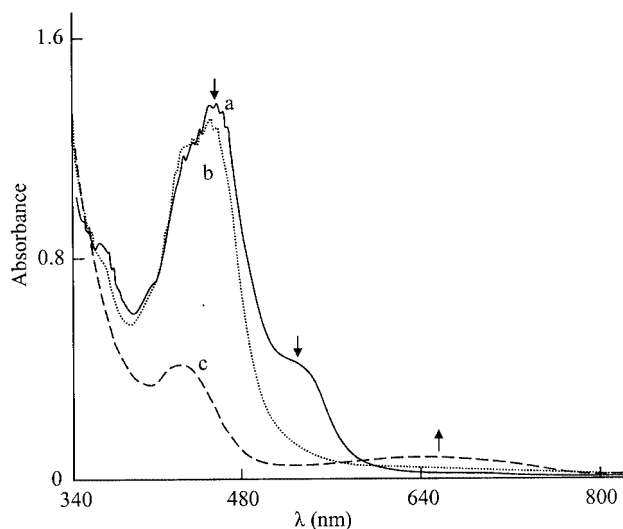
Figure 4. Absorption spectra of a 0.32 mM solution of [\{\text{Ru}(\text{LL}_4)\}_3\text{Fe}\}^{8+} in \text{CH}_3\text{CN} + 0.1 \text{ M Bu}_4\text{NClO}_4 : (a) initial solution, (b) after exhaustive electrolysis at 0.80 \text{ V} , (c) after exhaustive electrolysis at 1.10 \text{ V} ( l = 1 \text{ mm} ).
