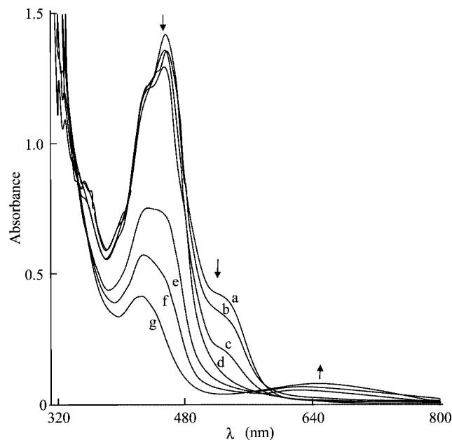
Figure 6. Spectral change of a mixture of [\{\text{Ru}(\text{LL}_6)\}_3\text{Fe}\}^{8+} (0.032 mM) and ArN 2 + (15 mM), under visible irradiation: (a) initial solution, (b) 3 s, (c) 12 s, (d) 24 s, (e) 120 s, (f) 220 s, (g) 700 s, ( l = 1 \text{ cm} ).
